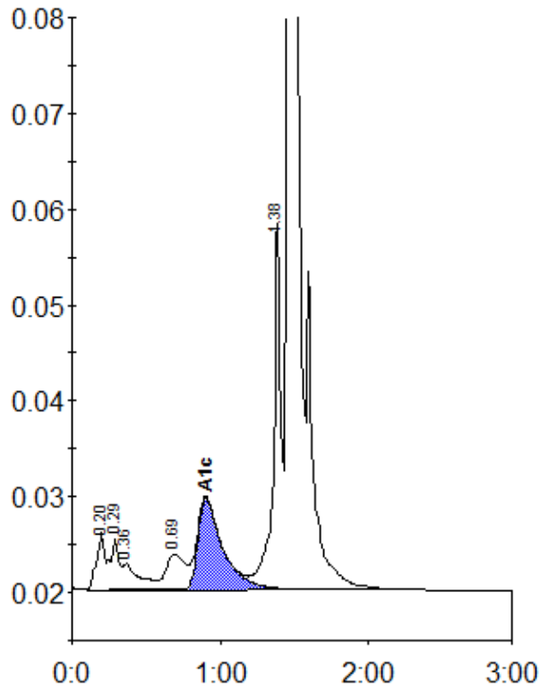
Peak table - ID: 10337077
